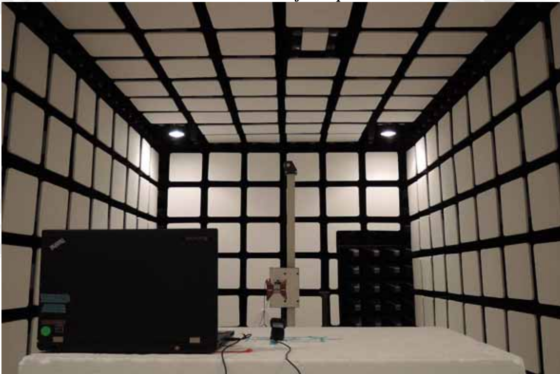
Back View of Set up
