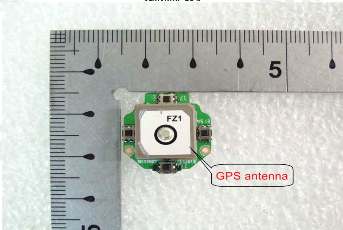
Antenna-GPS
